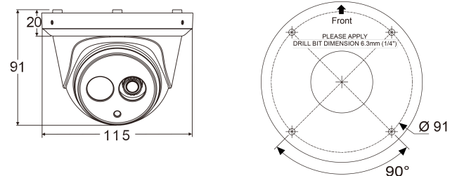
Dimension
