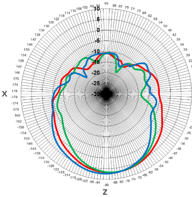
H Plane
