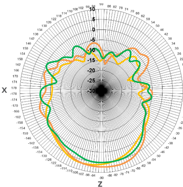
H Plane
