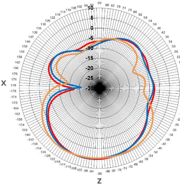
H Plane
