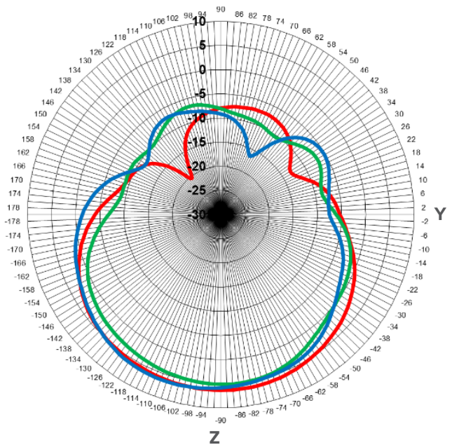
E Plane
