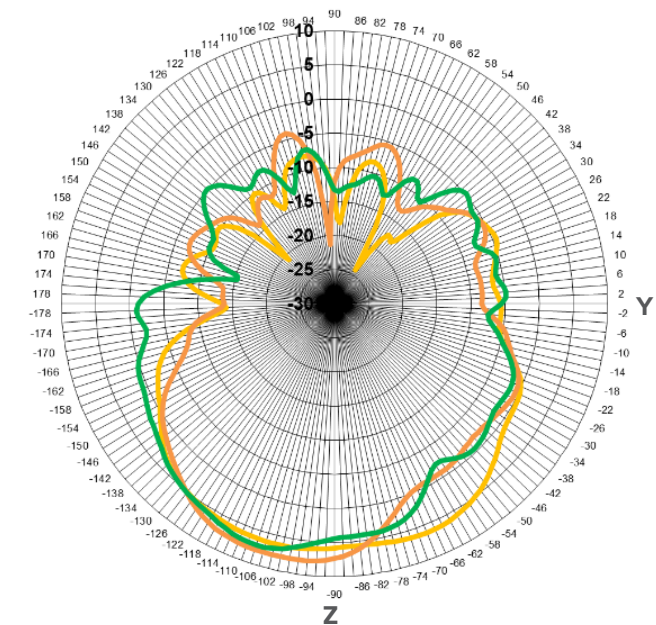
E Plane
