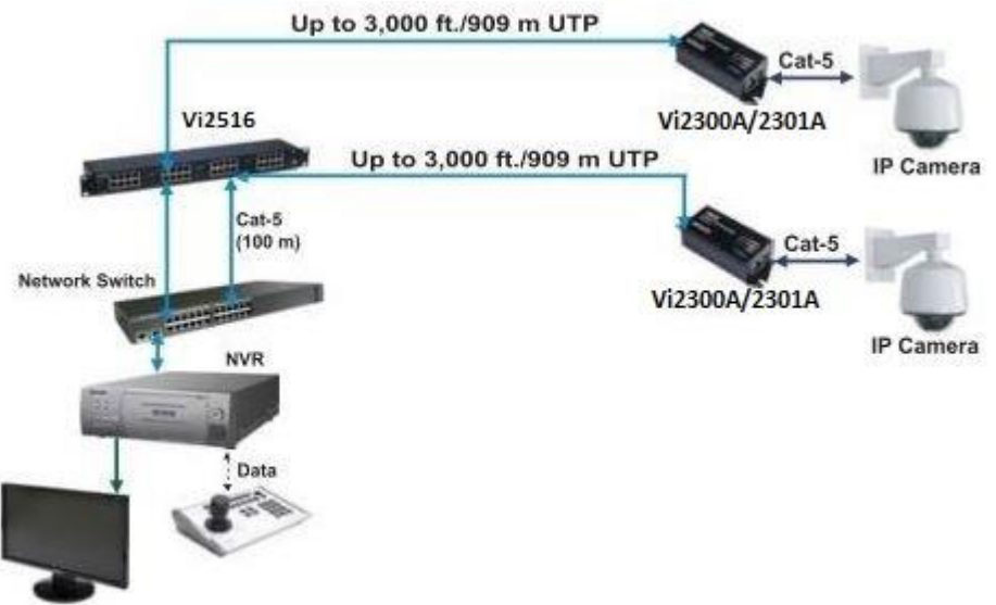
Figure 10: Vi2516 Application Drawing
