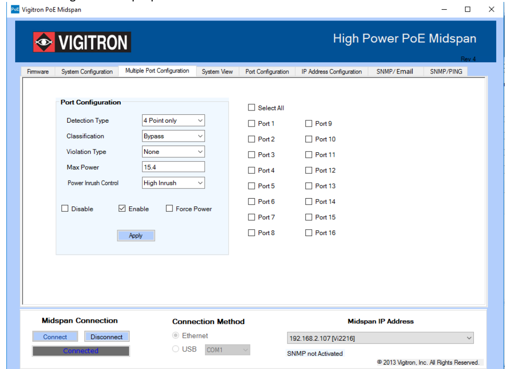
Figure 19: Multiple Port Configuration Window
