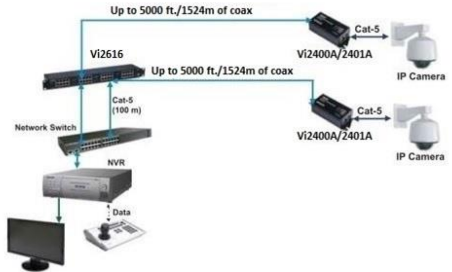
Figure 15: Vi2616 Application Drawing
