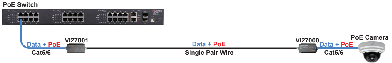
The Vi27000 series and a IP camera can be powered by a PoE switch.
