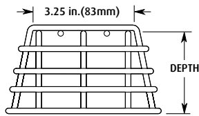
STI-9620 END VIEW
