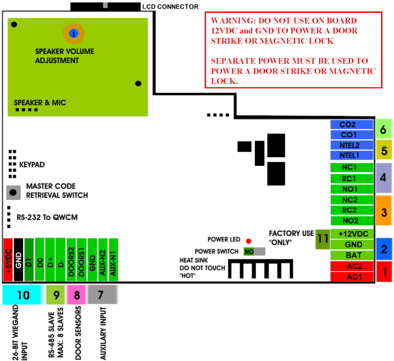
Figure 2.1 General Wiring Diagram
