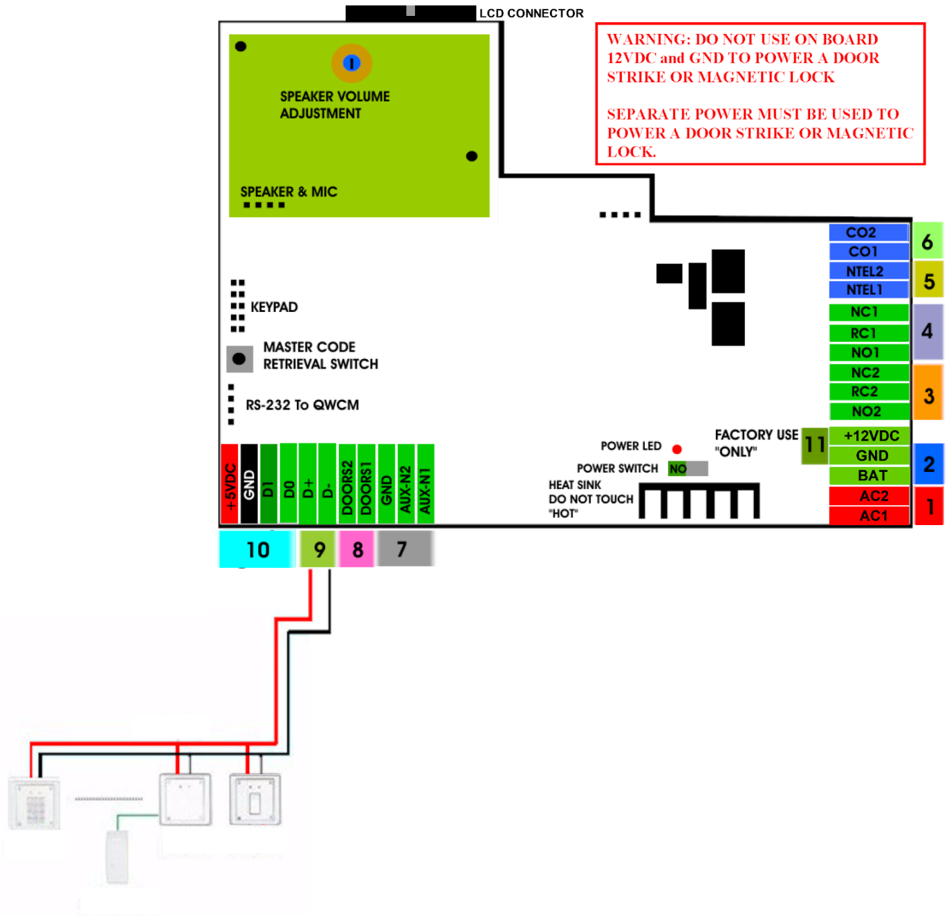
Figure 2.6 Satellite System Wiring Diagram
