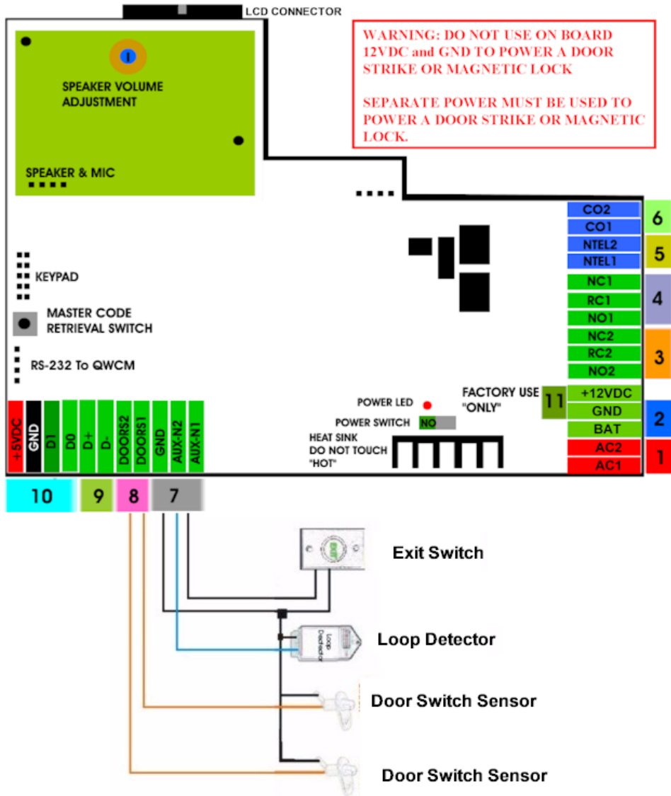
Figure 2.5 Input Device and Door Sensor Wiring Diagram
