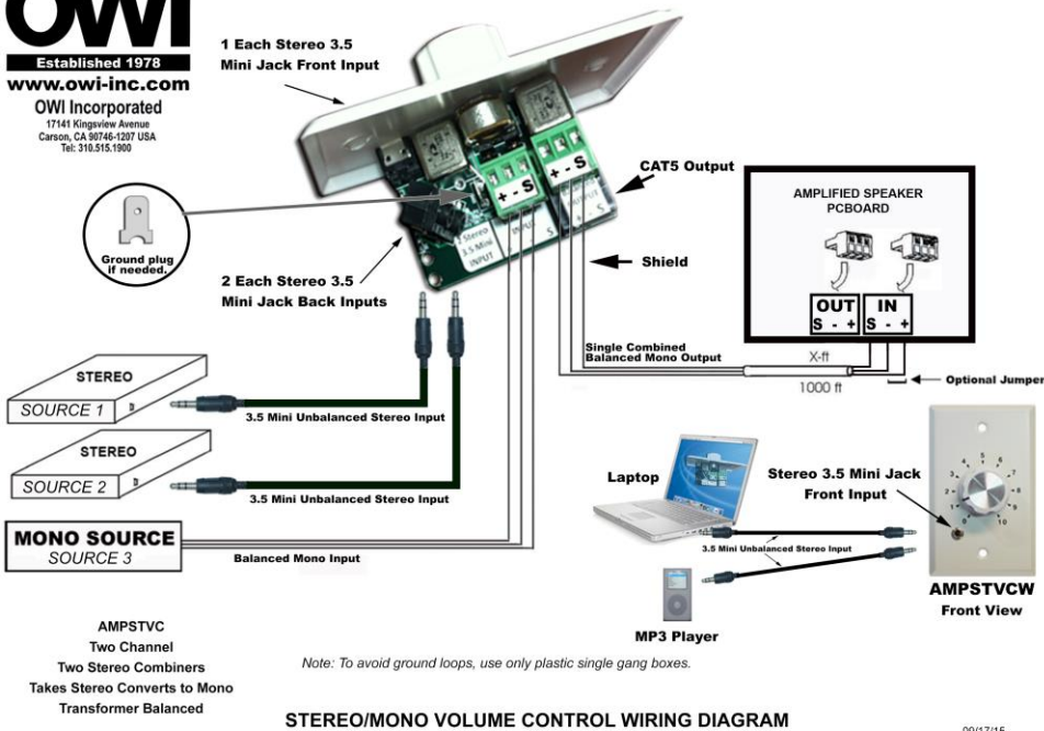
STEREO/MONO VOLUME CONTROL WIRING DIAGRAM
