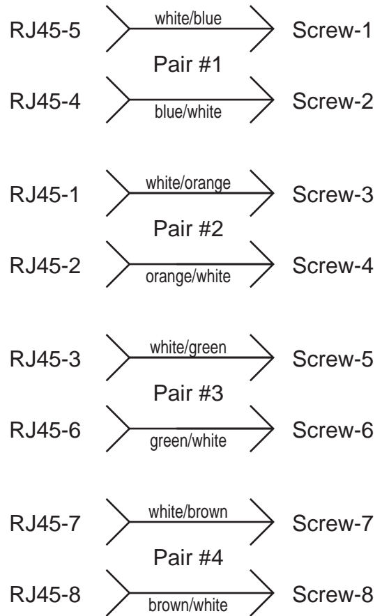
Schematic
