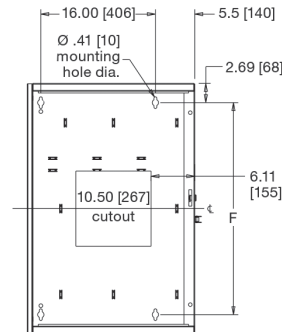
front view backpan
