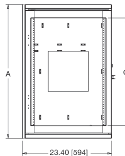
front view center section
