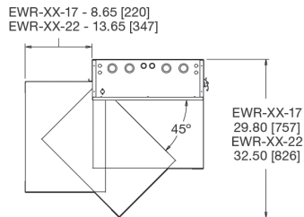
center section clearance
