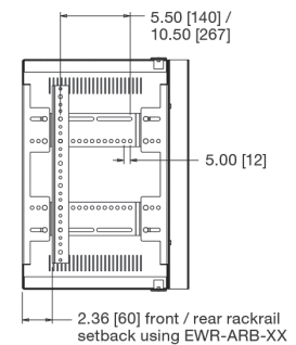
side view (shown with option EWR-ARB)
