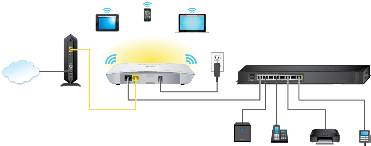
Figure 6. Set up the access point with a connection to your Internet modem
