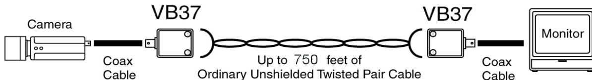
Basic Twisted Pair Video Transmission System
