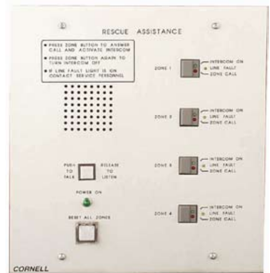
A-4204 4-zone Annunciator shown above 4 to 44 Zones Available
