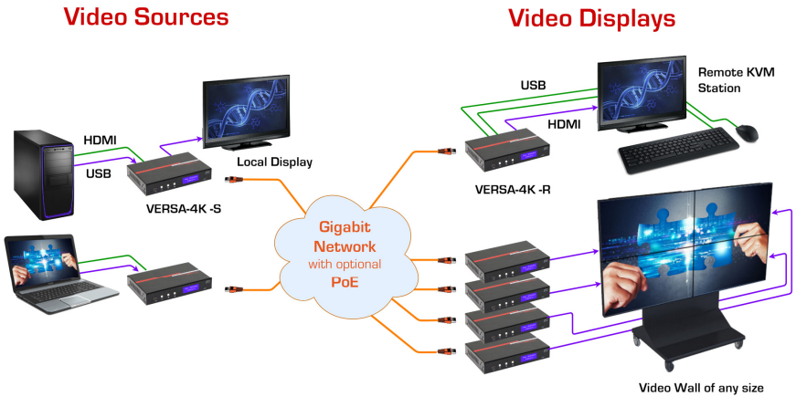
Fig 1: Block Diagram
