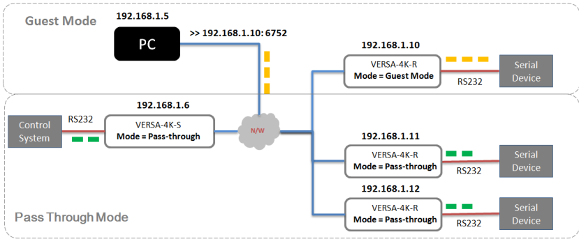
Fig 15. Serial Over IP
