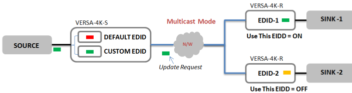
Fig 11. EDID Management
