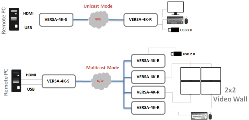
Fig 9: Unicast and Multicast Mode
