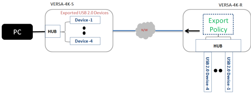
Fig 13. USB2.0 Export Policy
