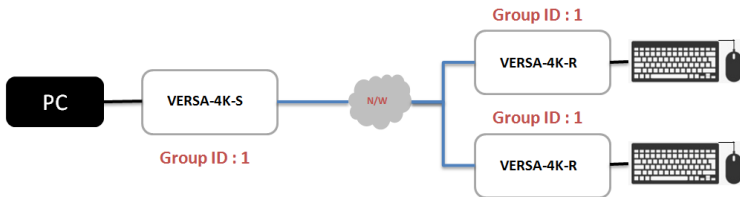
Fig 14. Keyboard and Mouse Over IP
