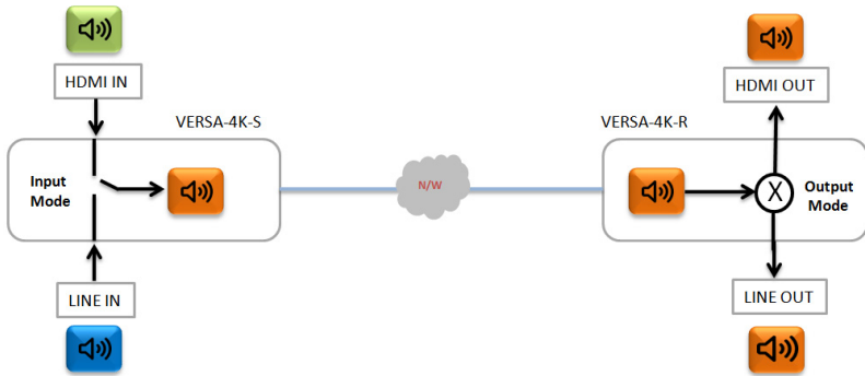
Fig 12. Audio Modes
