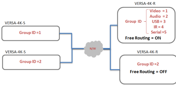
Fig 10. Independent Routing
