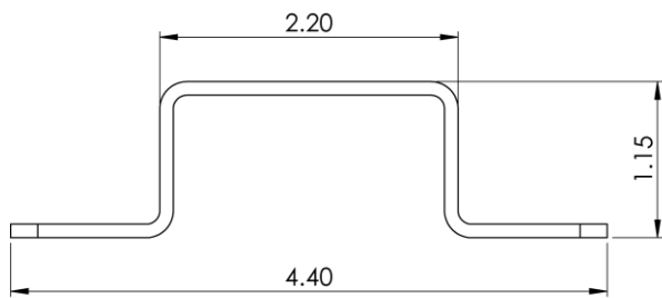
CEILING SUPPORT BRACKET
