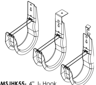
ICCMSJHK55- 4" J- Hook ICCMSJH955- 4" J- Hook with 90° Bracket ICCMSJHW55- 4" J- Hook with Bat Wing
