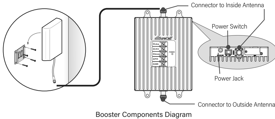
Booster Components Diagram
