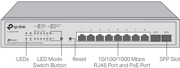
Figure 1-7 Front Panel of TL-SG2210MP
