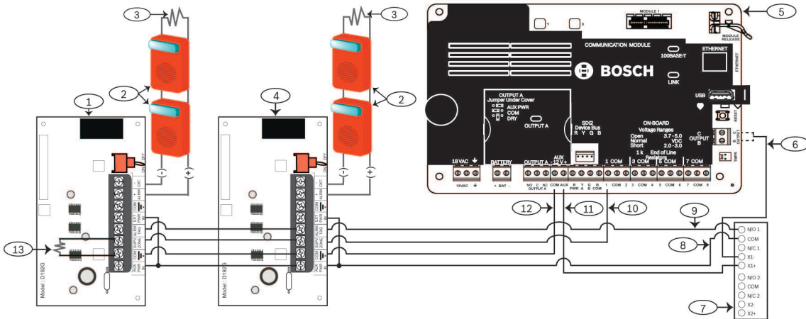
Figure 5.5: Wiring interconnected modules to a B Series panel supplying 12 VDC power
