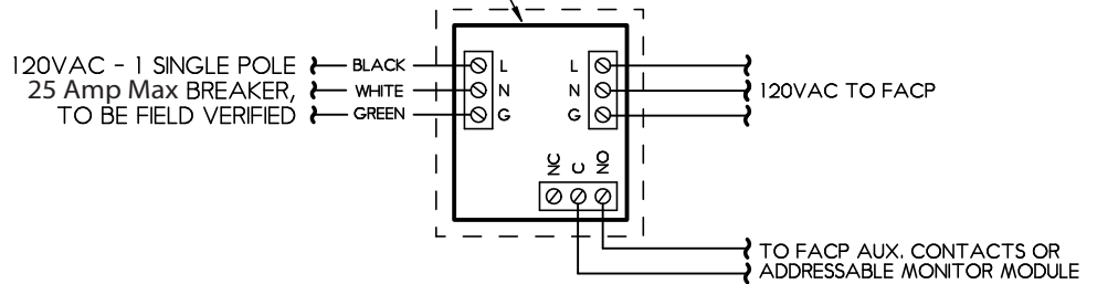
DTK-TSS4D SURGE PROTECTOR (TYPICAL)
