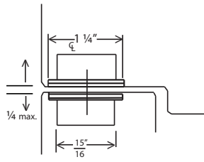
Overhead Installation, Side View
