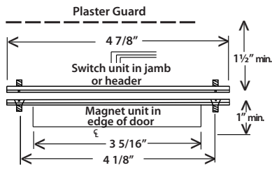
Overhead Installation, Front View
