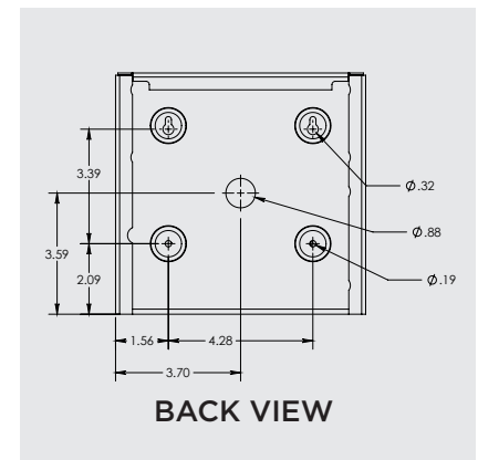
IP2501-d Dual Button Flush Mount
