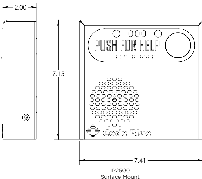
IP2500-s Single Button Surface Mount
