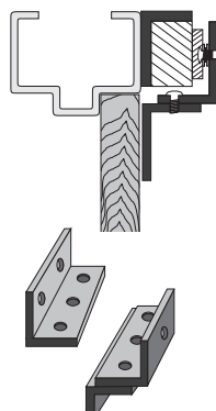
CX-1002/CX-1012 Set of L & Z Brackets
