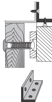
CX-1001/CX-1011 Adjustable L Bracket
