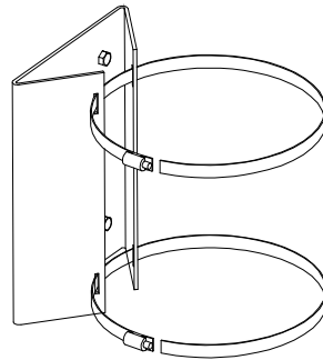
FIGURE 2-1: THREAD STRAPS THROUGH BRACKET
