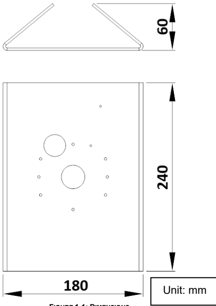
FIGURE 1-1: DIMENSIONS
