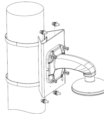
FIGURE 2-4: ATTACH WALL MOUNT TO POLE MOUNT
