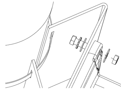
FIGURE 2-3: THREAD THE HEX BOLTS
