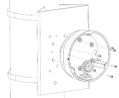
FIGURE 2-6: ATTACH BACK BOX TO POLE MOUNT
