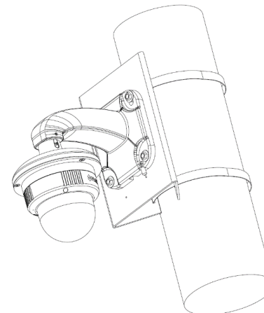
FIGURE 2-5: COMPLETED CM-3202 INSTALLATION
