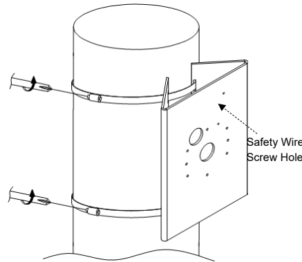
FIGURE 2-2: ATTACH KIT TO POLE
