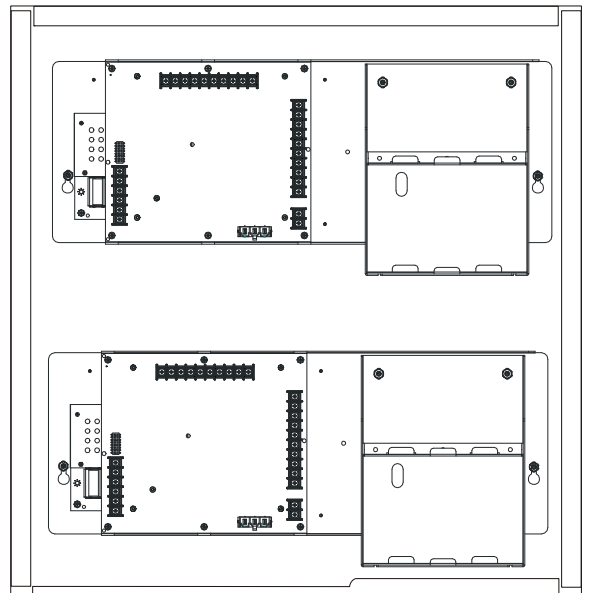
Figure 2.9 Two HPFF8CM Modules in an EQBB-B4 Cabinet (EQBB-B4 Backbox with EQDR-B4 Door)
