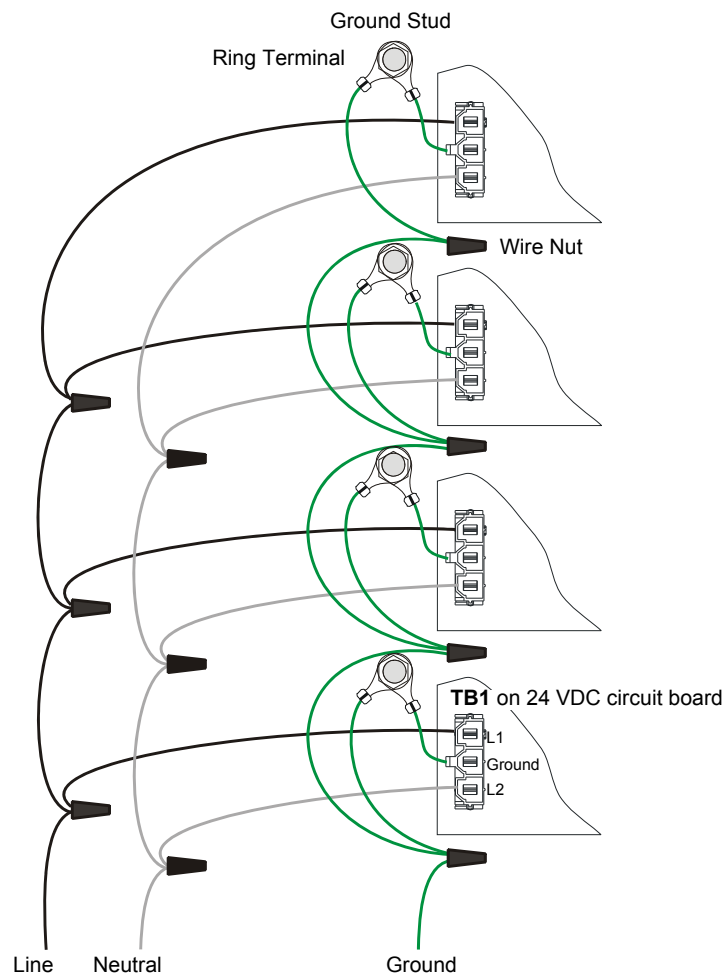
Figure 2.19 Nonpower-Limited Wiring Example: EQBB-D4 AC Wiring (Expanded)
