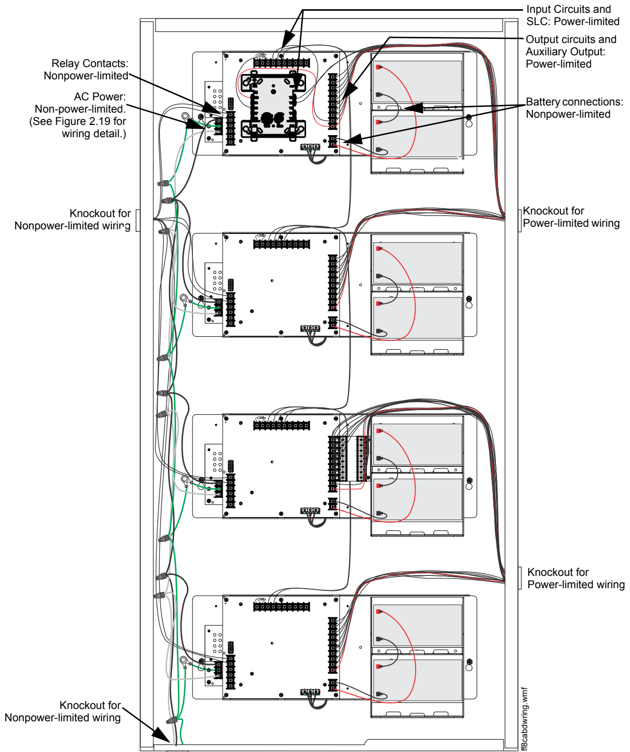
Figure 2.18 Power-Limited Wiring Example: EQBB-D4
