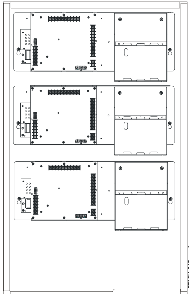
Figure 2.6 Three HPFF8CM Modules in a CAB-C4 Cabinet (SBB-C4 Backbox with DR-C4 Door)
