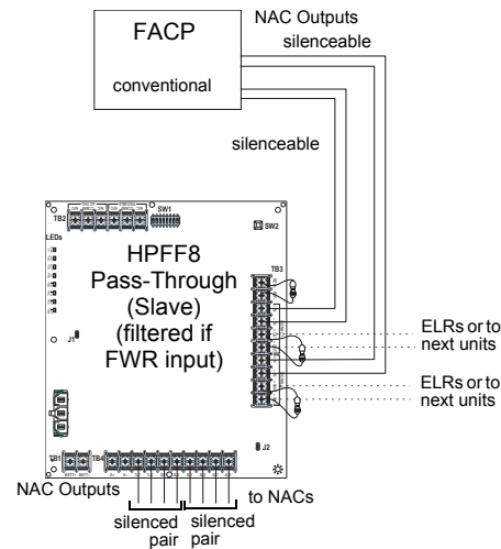
Figure 5.10 Selective Silencing Connections
