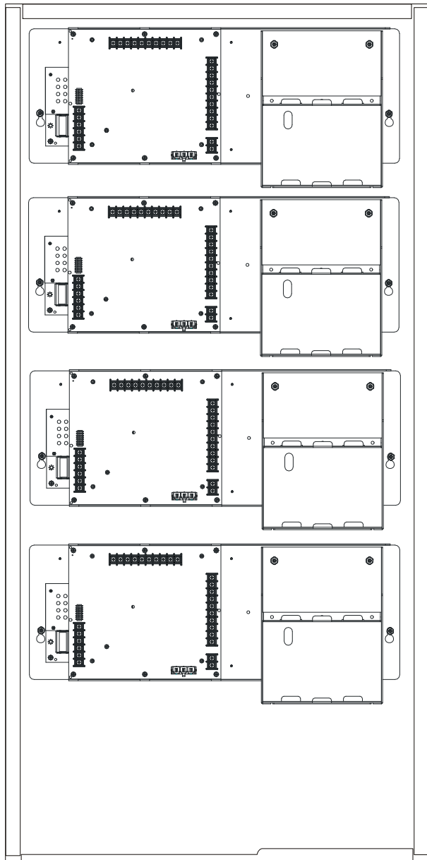
Figure 2.5 Four HPFF8CM Modules in a CAB-D4 Cabinet (SBB-D4 Backbox with DR-D4 Door)
