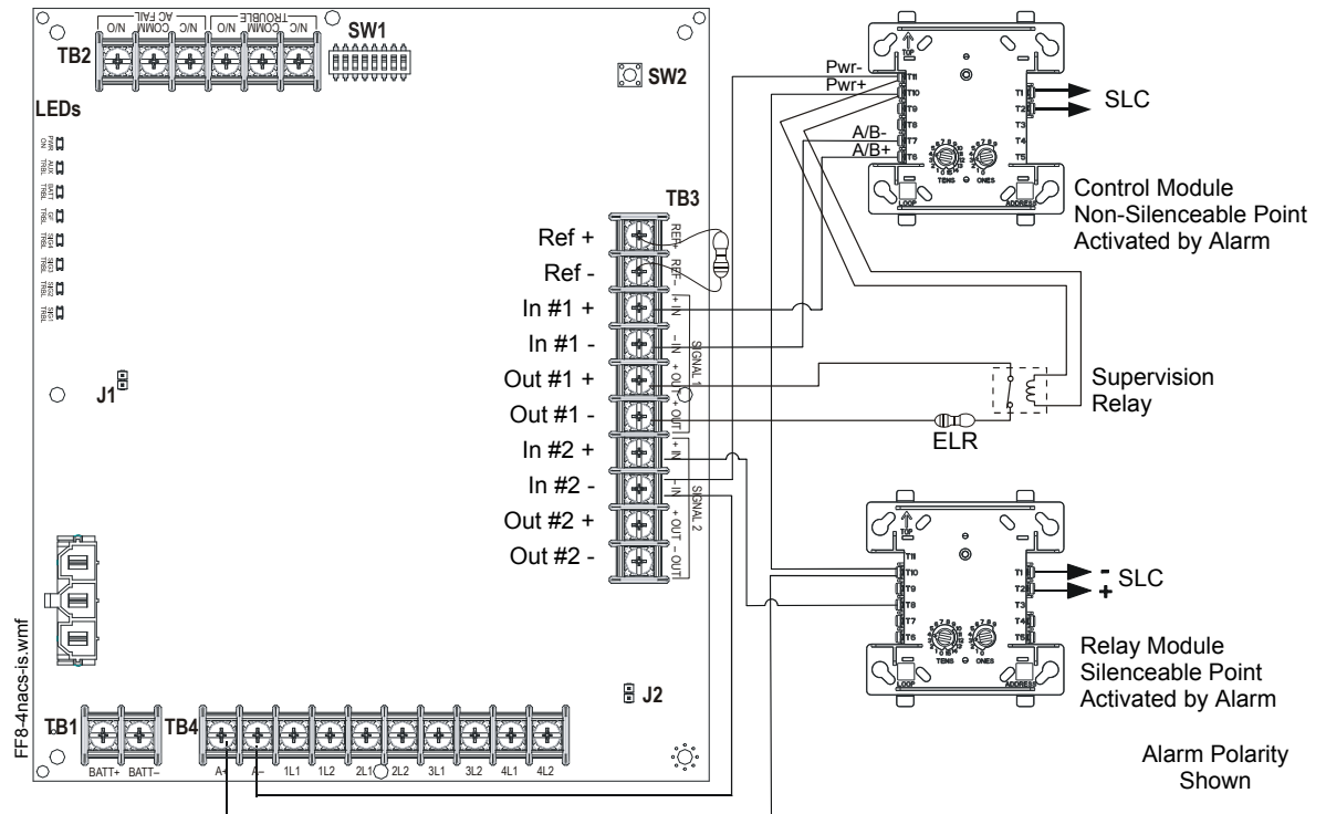
Figure 5.2 Controlling and Silencing Four NACs
