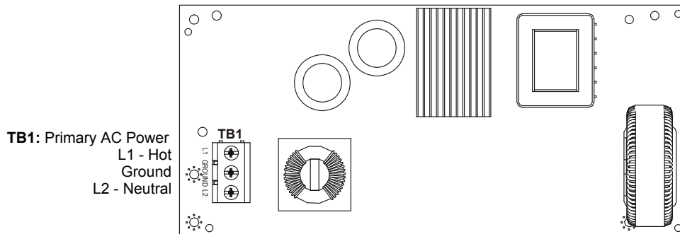
Figure 1.2 HPFF8 24 VDC Power Supply Circuit Board
