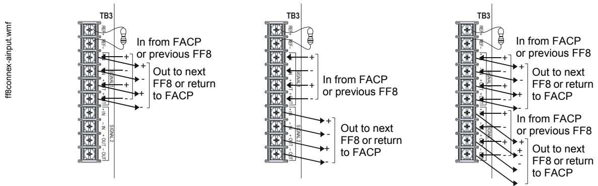
Figure 5.8 Class A Input Connections
