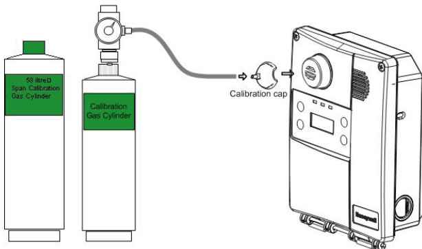
Figure 9. Calibration Installation
