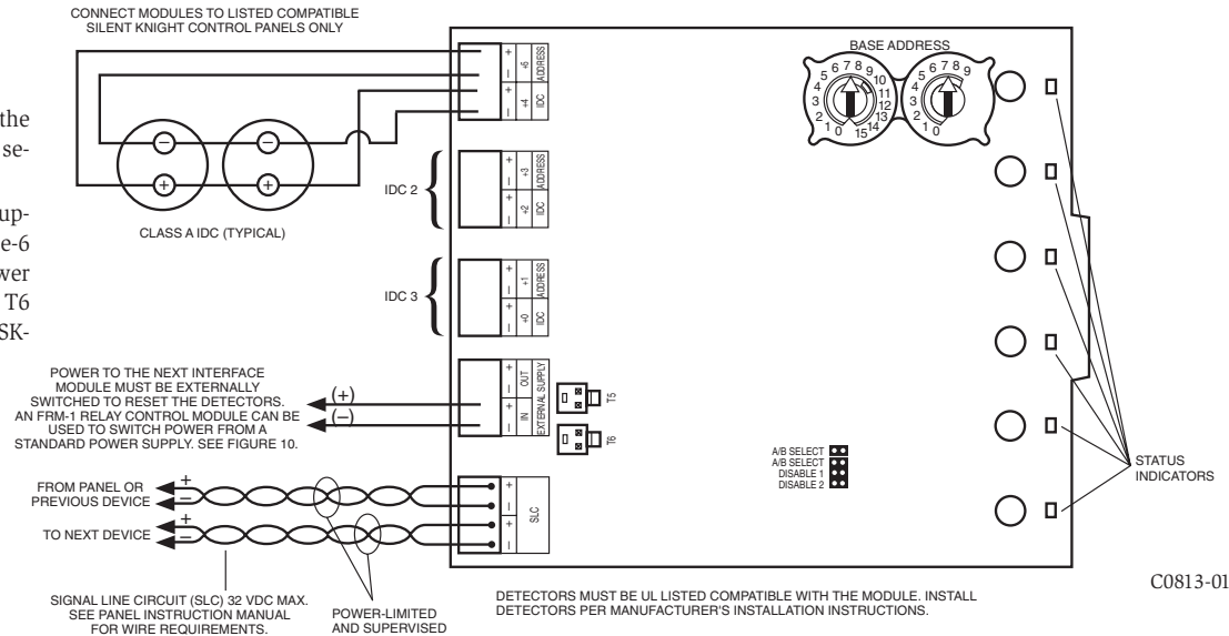
FIGURE 6: INTERFACE TWO-WIRE CONVENTIONAL DETECTORS – CLASS A, STYLE D.
