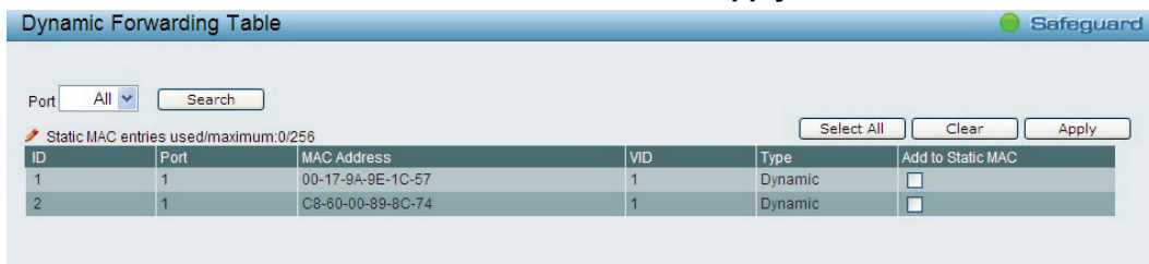
Figure 4.47 – L2 Functions > MAC Address Table > Dynamic Forwarding Table
