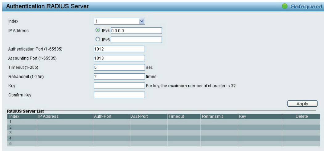
Figure 4.95 – AAA > RADIUS Server
