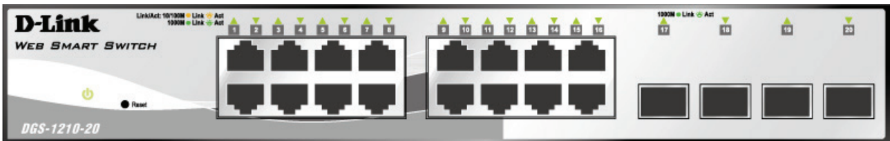
Figure 1.5 – DGS-1210-20 Front Panel
