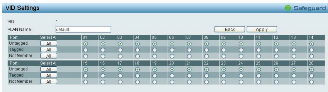
Figure 4.36 – Configuration > 802.1Q VLAN > Add VLAN
