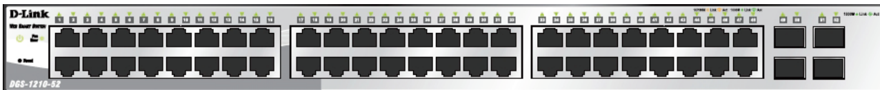
Figure 1.11 – DGS-1210-52 Front Panel
