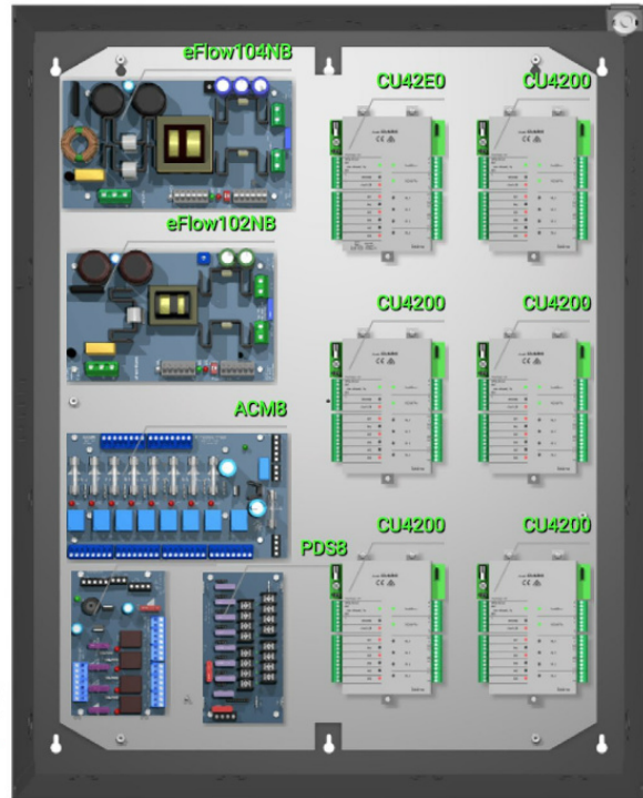
T2SAK75F12 12-Door Access System with Power
