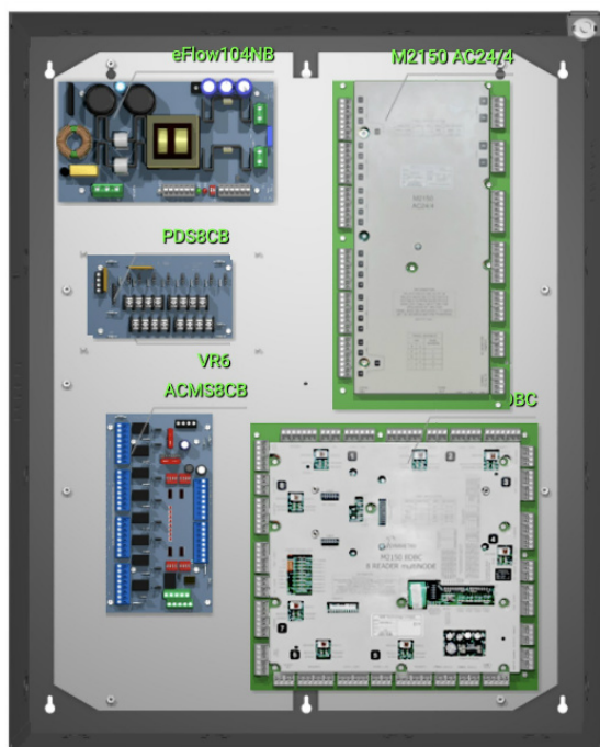
T2AGK2 12-Door Access System with Power
