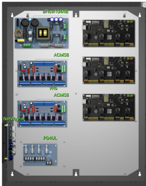
T2SFK7F16S 12-Door Access System
