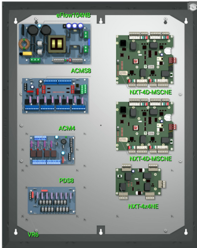
T2KSK7F12 12-Door Access System with Power
