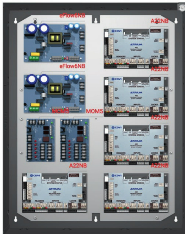
T2CVK33F10 10-Door Access System with Power
