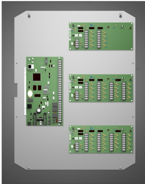
T2MK3F8Q with TDMD2 8-Door Access System with Power + Network Power Management with DMP Intrusion Door Backplane
