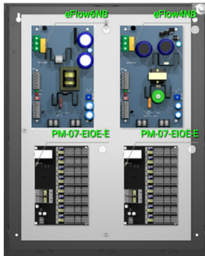
16-Door Access System with Power
