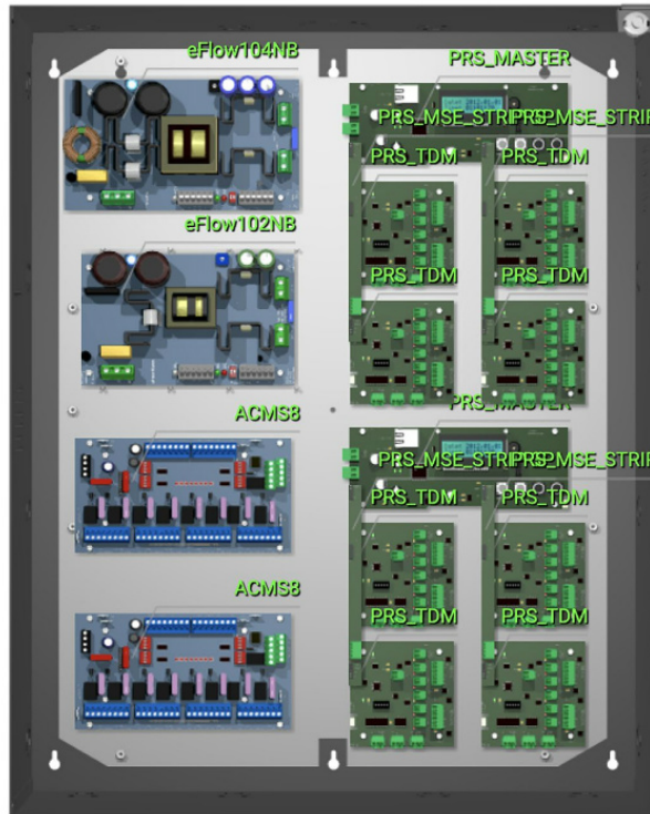
T2HCK75F16 16-Door Access System with Power
