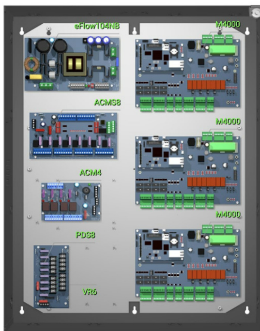
T2AGK2 12-Door Access System with Power
