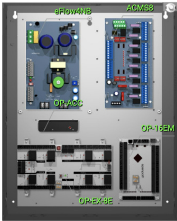
T1PHK3F8 8-Door Access System with Power and Elevator Control
