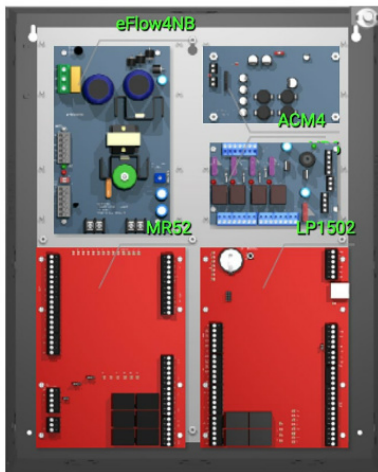
T1MK1F4 4-Door Access System with Power
