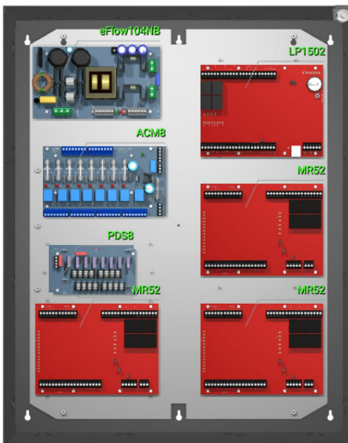
T2MK7F8 8-Door Access System with Power
