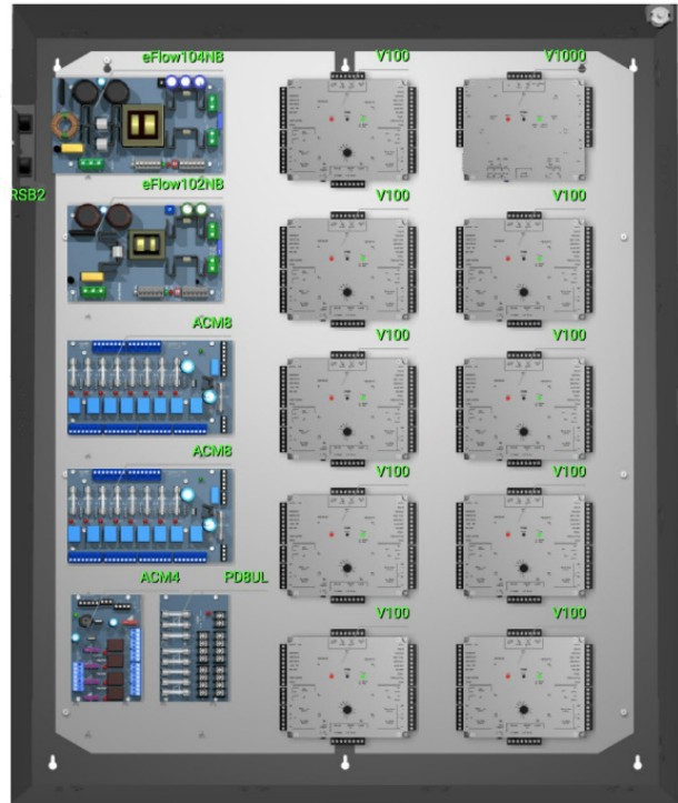
T3VK75F20 20-Door Access System with Power
