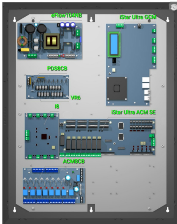
T2SK7F8D 8-Door Access System with Power
