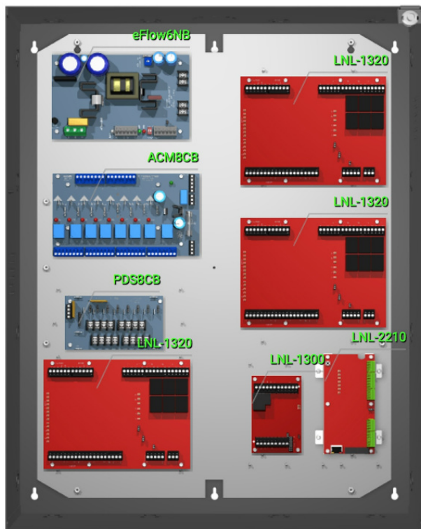
T2MK3F8D 8-Door Access System with Power
