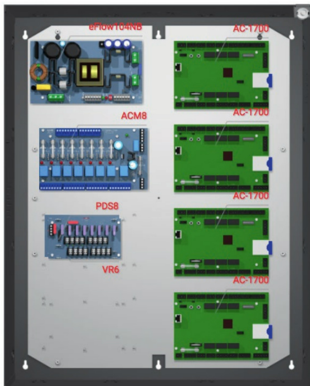
T2SLK7F8 8-Door Access System with Power
