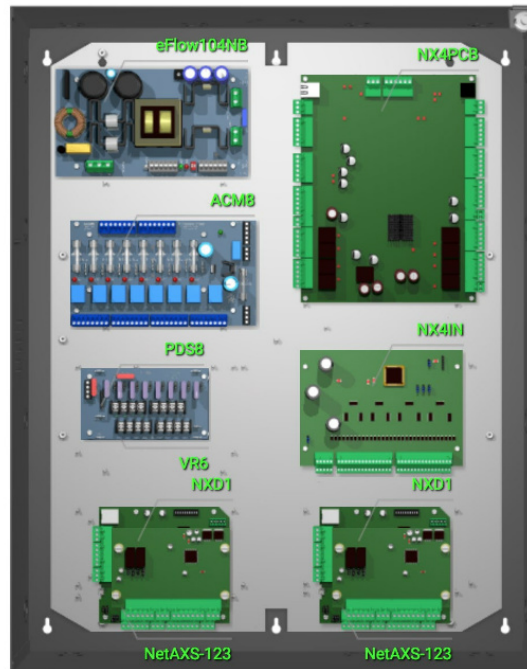
T2HNK7F8 8-Door Access System (NetAXS) with Power
