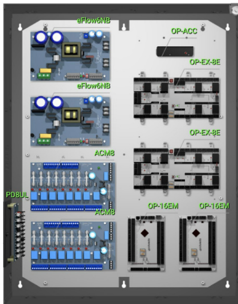
T2PHK33F16 16-Door Access System with Power and Elevator Control
