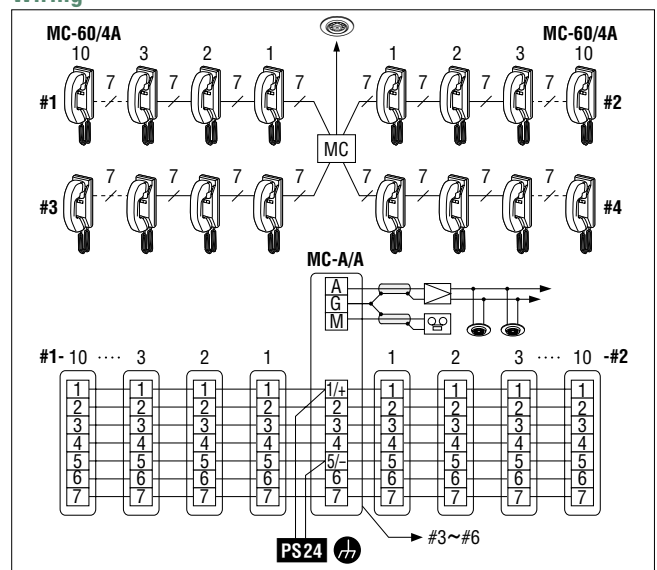
Station blocks #1~6 of max. ten MC-60/4A's
