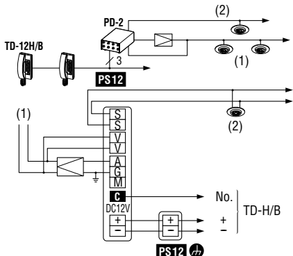
(1) Paging Speakers (2) Talkback speakers PS12 : PS-1225S, PS-1225UL, PS-1225BF, PS-1225DM, PS-1225
