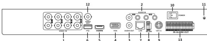
DS-7208HTI-K2
