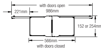
dual duct dimensions
