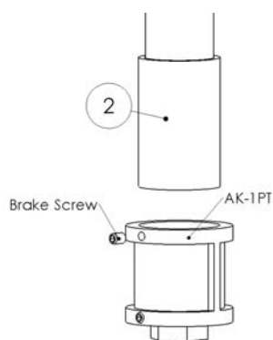
Step 2: Securing the outer mast
