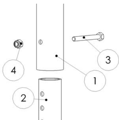
Step 4: Attaching the two masts
