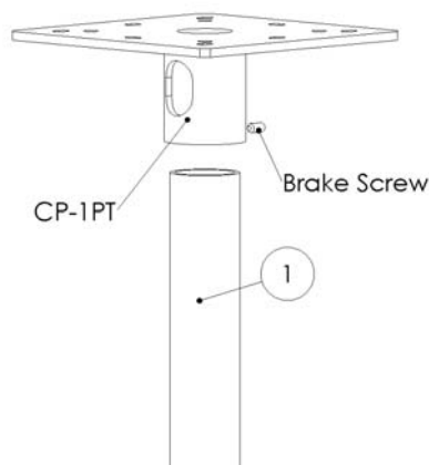
Step 2: Securing the outer mast
