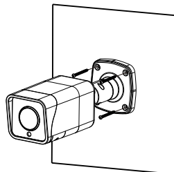
Figure 3-2 Installing camera
