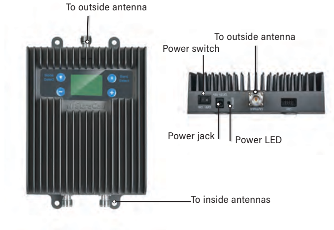
Host unit diagram
