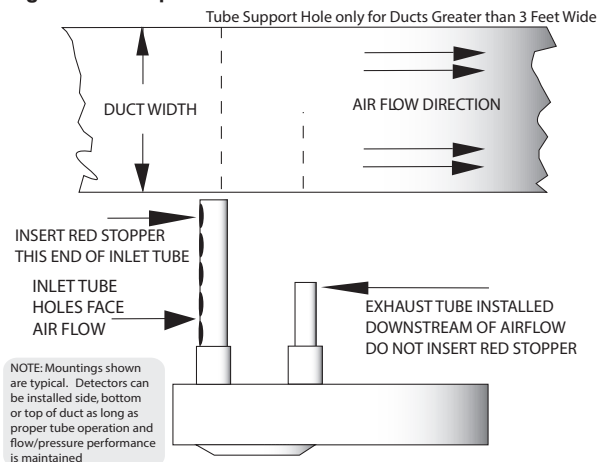
Figure 4. Example of the PAD200-DUCT Duct Detector Placement
