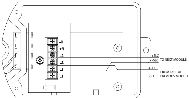
Figure 3. Example of Wiring a PAD200-DUCT Duct Detector
