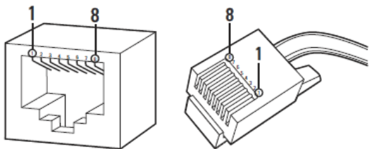
Figure 10. Pin Numbering
