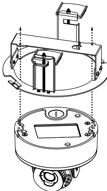
Figure 6. Attaching the Back Box to the In-Ceiling Mounting Bracket
