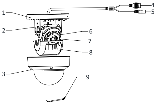
Figure 1-4 Overview Of Type V Camera
