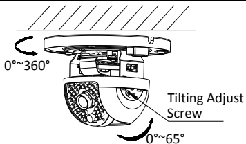
Figure 2-6 Angle Adjustment of Type I Camera
