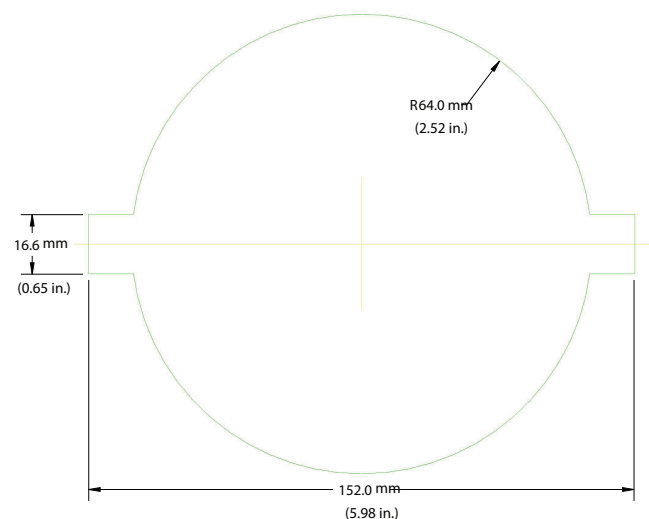
Ceiling hole cut-out dimensions
