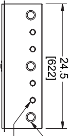
TOP VIEW
