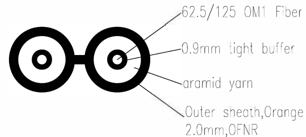
∅2.0mm OFNR cable section
