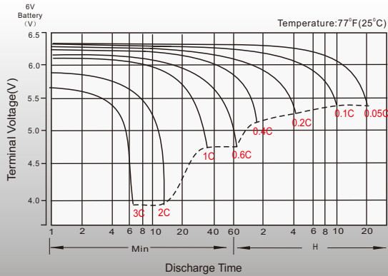
Curves represent Constant Current draw (Amp.) 1C curve = 1 x Nominal capacity = 1.2amp. constant draw 0.05C curve = 0.05 x Nominal capacity = 0.06amp. draw
